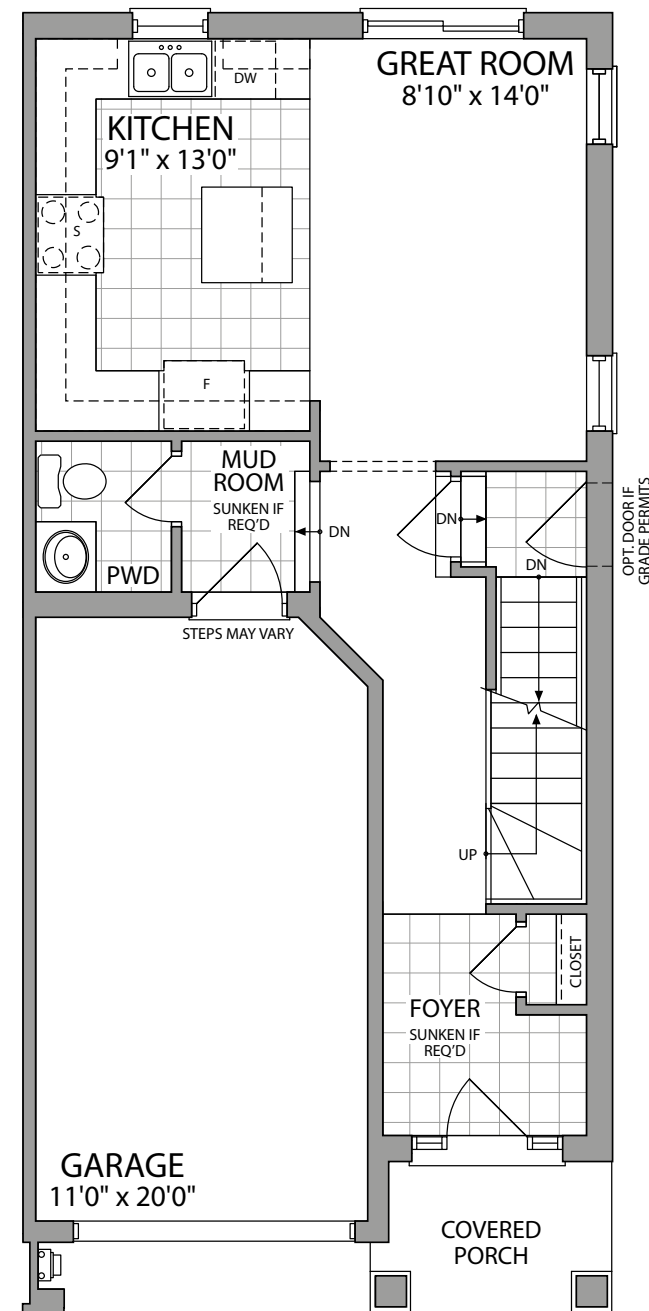
GROUND FLOOR ELEVATION A & B
