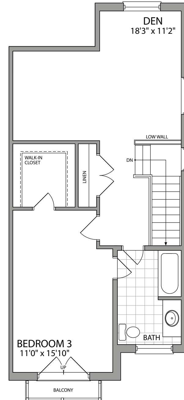
THIRD FLOOR ELEVATION A
